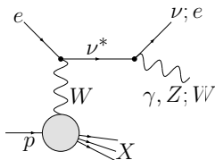
Excited neutrinos
